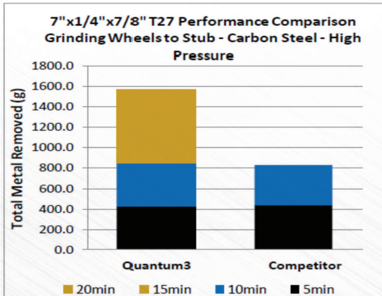
Figures 2 and 3 represent the performance of 7" and 9" Grinding Wheels for both Norton Quantum3 and 3M CUII. Wheels were ground to Stub using Carbon Steel as the material application measuring at 5 minute intervals.
